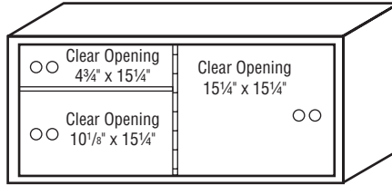
ATL-3R Weight (Lbs): 255 (MFG. #9035030) Retail: $1,625
